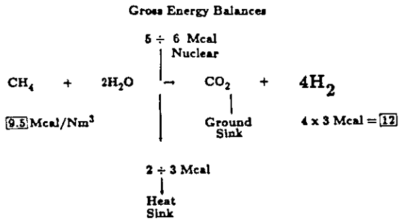
Fig. 11. A skeleton description of the steam reforming process with the help of nuclear heat is here given to show the energy balances. Basically, reforming adds about 30% to methane's energy input. This extra energy obviously comes from the nuclear heat, with an efficiency of 50% or more. This process appears relatively simple and very suited to introduce large amounts of nuclear energy into the fuel system.
