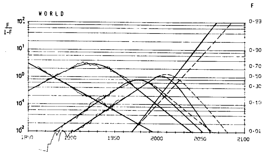
Fig. 11. Effect of an accelerated nuclear program (solid lines). Again only gas consumption appears to be heavily affected.
