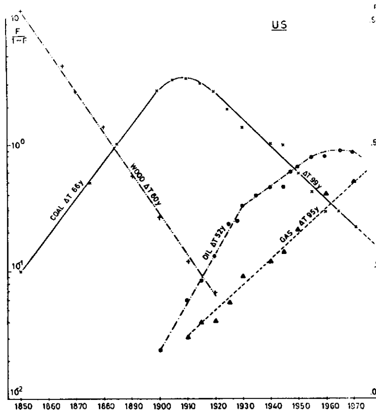
Fig. 5. Fitting of the statistical data on primary energy consumption in the U.S. Straight lines are represented by equations of type (2). Rates of penetration are indicated by the time to go from 1% to 50% of the market ( \Delta T years). The knee in the oil curve and the saturation regions can be calculated by the rule "first in—first out".
