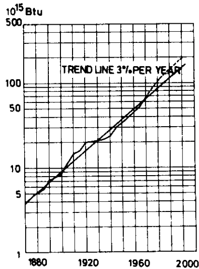
Fig. 2. U.S. energy consumption including wood and farm waste. The trend line has a 3% slope. (Adapted from R.E. Lapp, The Logarithmic Century .)
