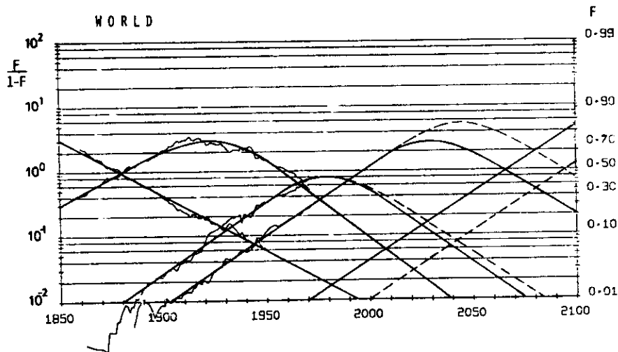
Fig. 10. The effects of the moratorium shown by respect to the base case. Penetration of nuclear energy is taken very prudently to be about 4% in year 2000.
