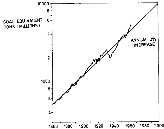
Fig. 1. World energy consumption, including wood and farm waste. The trend line has a 2% slope.
