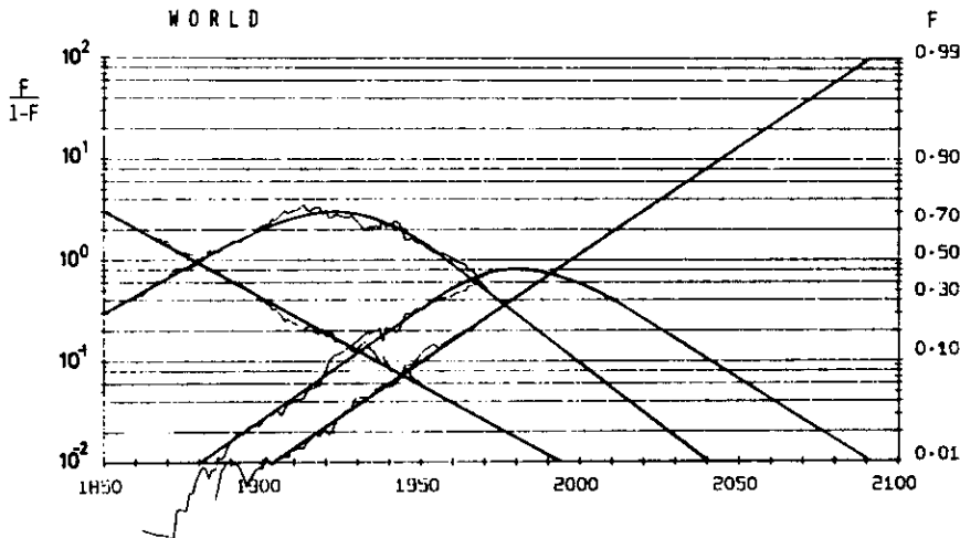
Fig. 8. The assumption that no nuclear energy, or new sources will be introduced leads to the absurd situation where all energy input will rely on natural gas.
