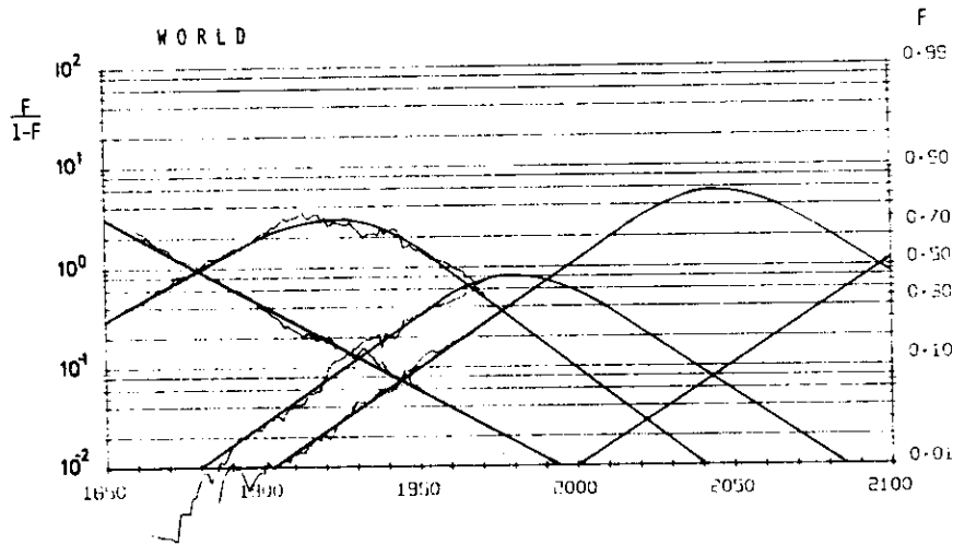
Fig. 9. Even the assumption of a moratorium for nuclear energy up to the year 2000 leads to a situation of incompatibility with gas resources. The introduction of nuclear energy appears a perfectly timed device to make ends meet.
